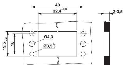
Mounting cutout
