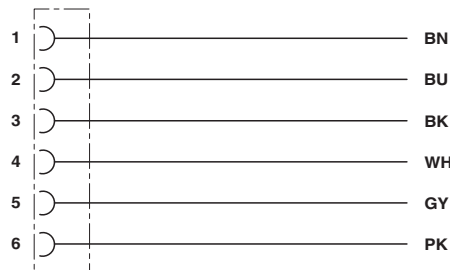
Contact assignment of the DEUTSCH DT06-6S
