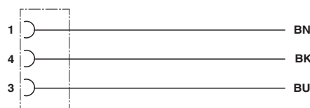
Contact assignment of the M12 socket
