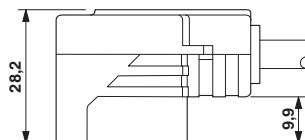
Dimensional drawing
