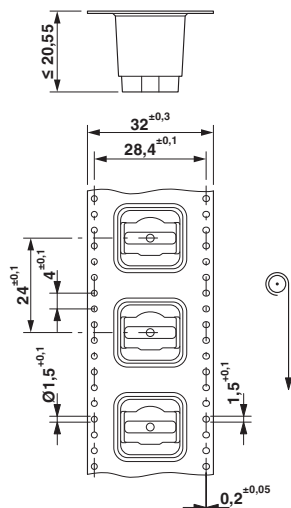
Dimensional drawing
