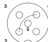
Pin assignment socket M 12, 3-pos. + PE
