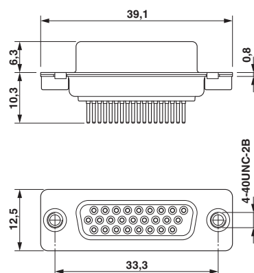
Dimensional drawing
