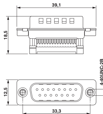
Dimensional drawing
