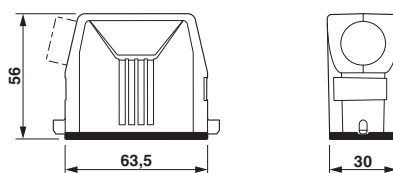
Dimensional drawing
