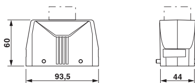
Dimensional drawing
