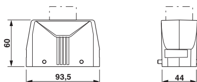
Dimensional drawing
