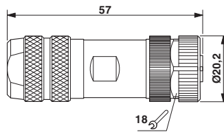
Dimensional drawing
