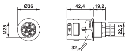
Dimensional drawing of QPD W 4PE6,0 M25
