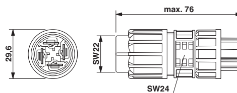
Dimensional drawing: connector, 2.5 mm 2
