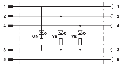
Contact assignment of M12 plugs / sockets with 3 LEDs
