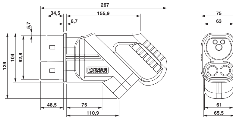
Dimensional drawing
