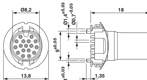
M12 female contact carrier, straight
