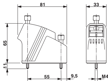
Dimensional drawing
