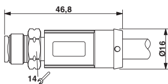
Plug, M12 x 1, straight, shielded
