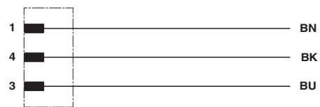
Contact assignment of the M12 plug
