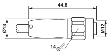
Dimensional drawing
