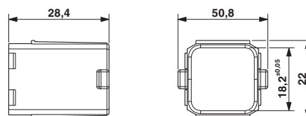
Dimensional drawing
