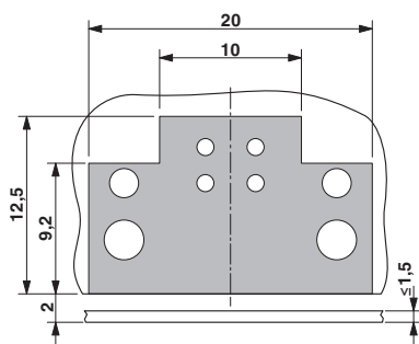
Dimensional drawing
