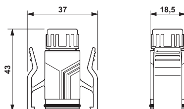
Dimensional drawing
