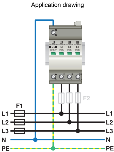
Figure shows version with remote indication contact
