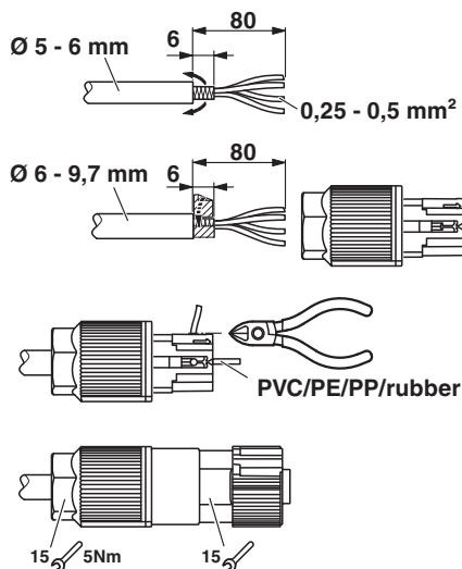
Dimensional drawing
