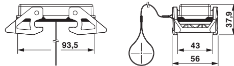
Dimensional drawing
