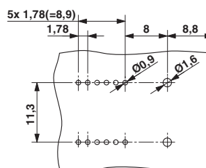
Drilling diagram
