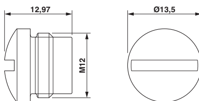
Dimensional drawing
