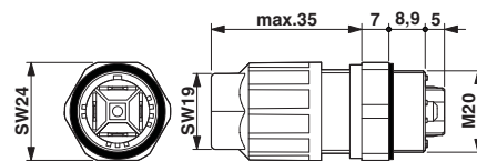
Dimensional drawing
