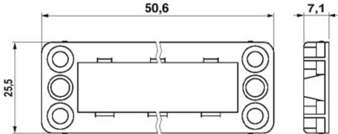
Dimensional drawing
