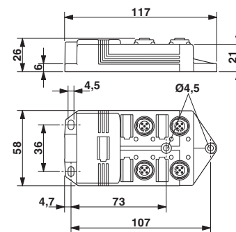
Dimensioned drawing
