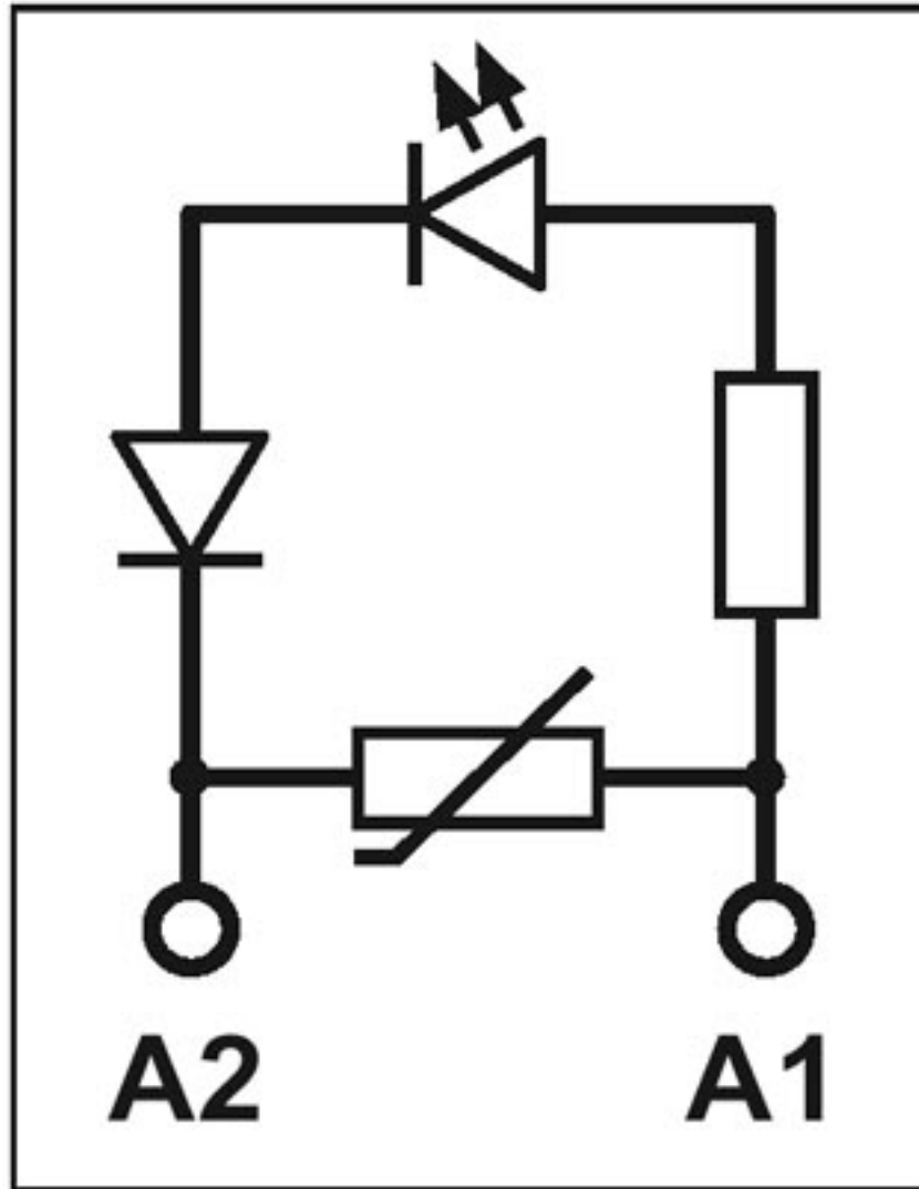
Circuit diagram
