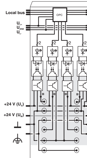
Block diagram
