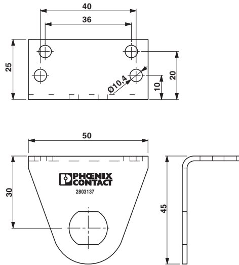
Dimensioned drawing
