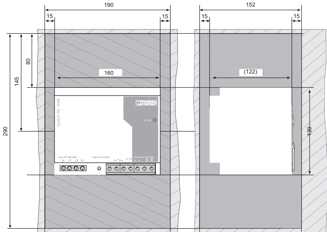
Dimensioned drawing
