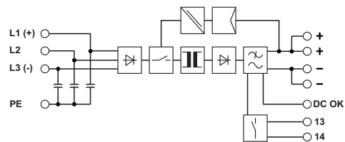
Product drawing
