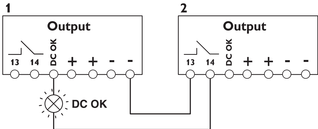
Circuit diagram
