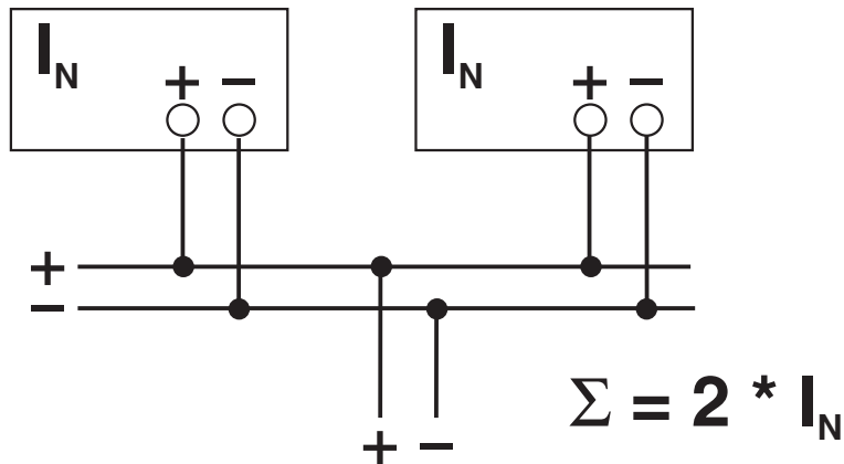
Circuit diagram
