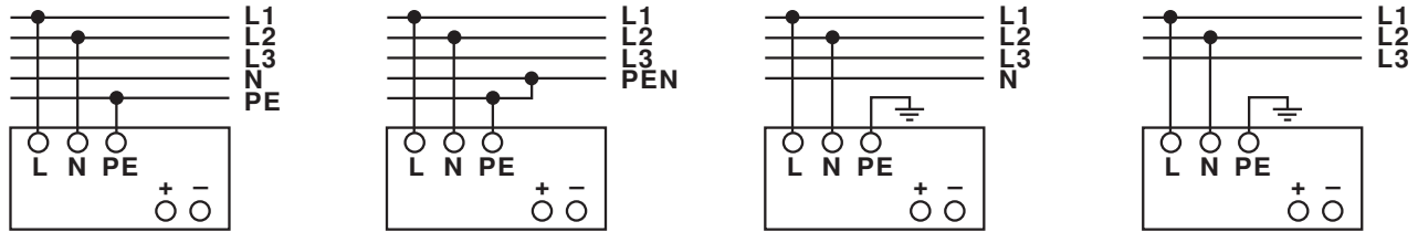
Connection diagram
