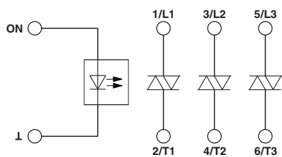
Block diagram
