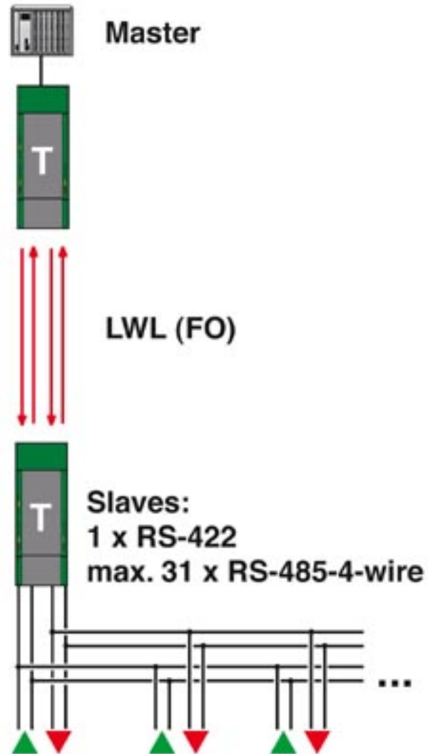
Application drawing
