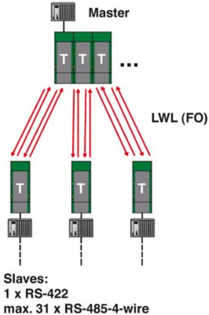
Application drawing
