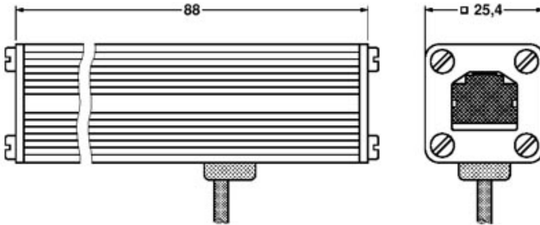
Dimensioned drawing
