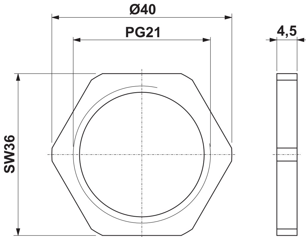
Dimensioned drawing
