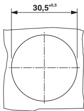
Dimensioned drawing
