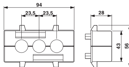
Dimensioned drawing
