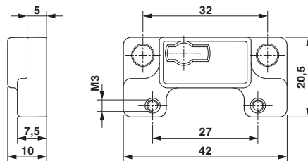
Dimensioned drawing
