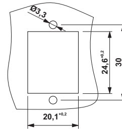
Dimensioned drawing
