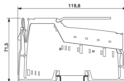
Dimensioned drawing
