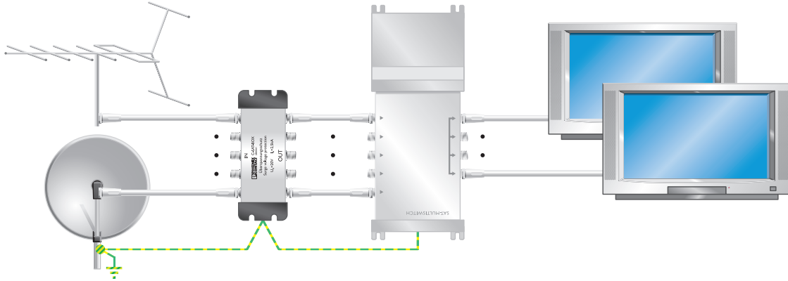
Application drawing
