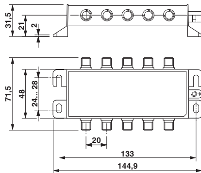
Dimensioned drawing
