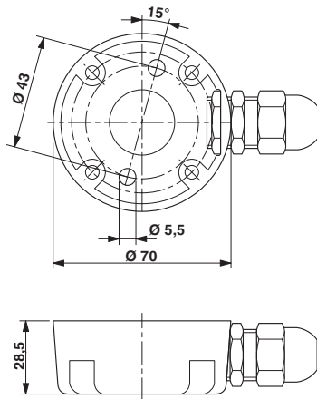
Dimensioned drawing
