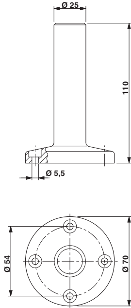
Dimensioned drawing
