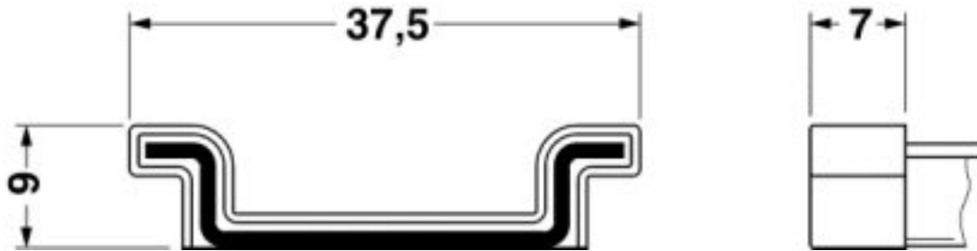
Dimensioned drawing
