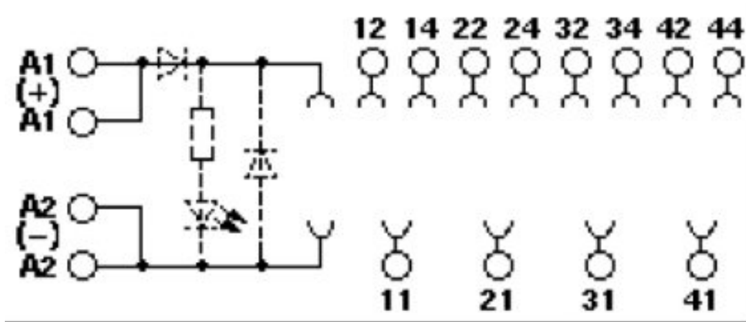
Circuit diagram
